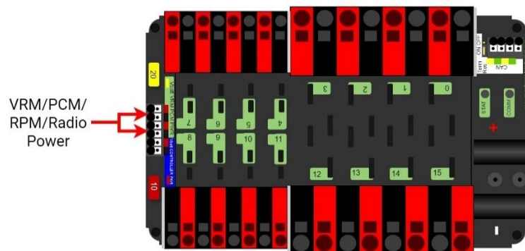
Figure 8-13 VRM, PCM, RPM, and Radio power source on a PDP
