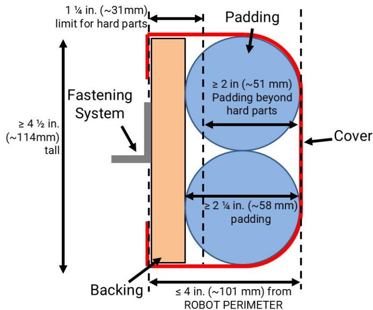
Figure 8-5 BUMPER Cross Section Example
