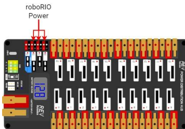
Figure 8-10 roboRIO power source on a PDH
