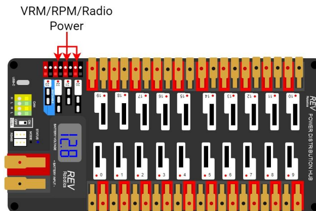
Figure 8-14 VRM/RPM/Radio power source on a PDH
