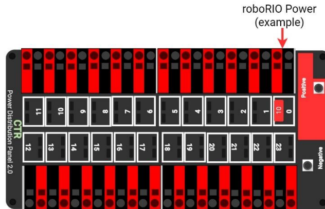
Figure 8-11 roboRIO power source on a PDP 2.0
