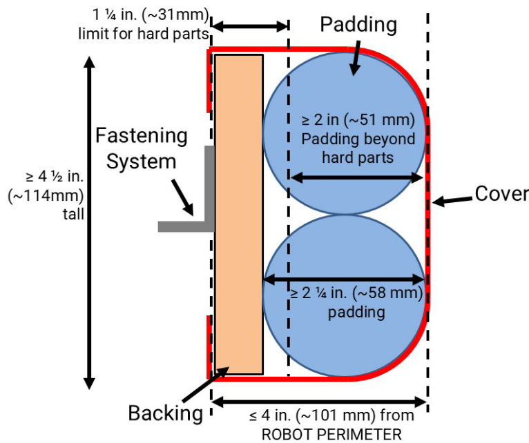
Figure 8-5 BUMPER Cross Section Example
