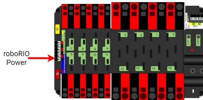
Figure 8-9 roboRIO power source on a PDP
