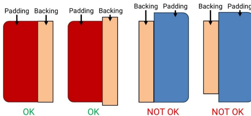
Figure 8-4 BUMPER backing supporting padding
