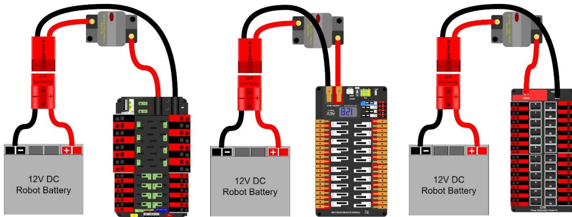
Figure 8-8 Electrical connection diagram
