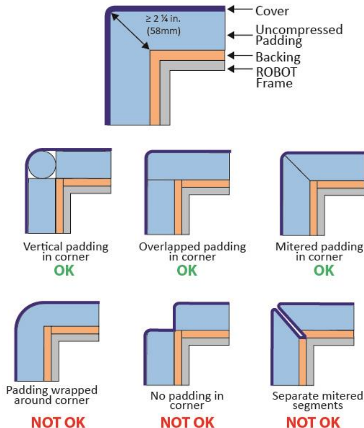
Figure 8-7 Uncompressed corner padding
