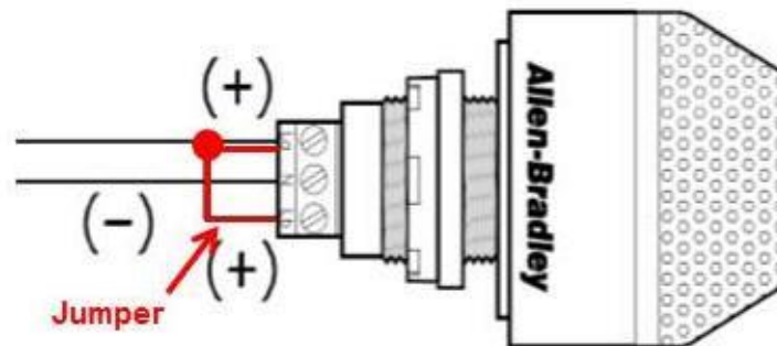
Figure 8-16 855PB-B12ME522 jumper wiring
